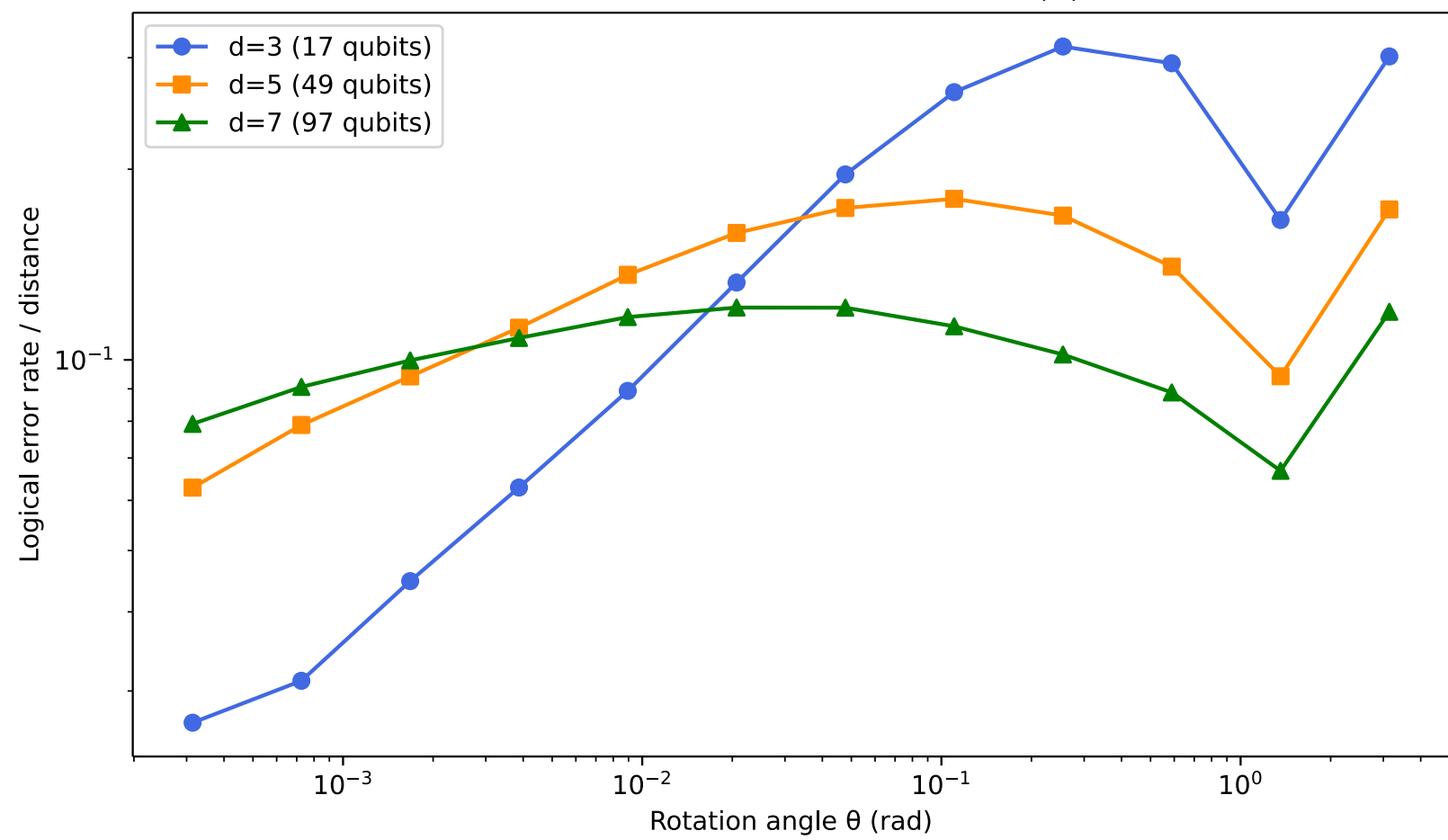
STAR Fidelities — Surface Code d=3,5,7
